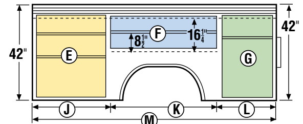
"A" Compartment Layout
