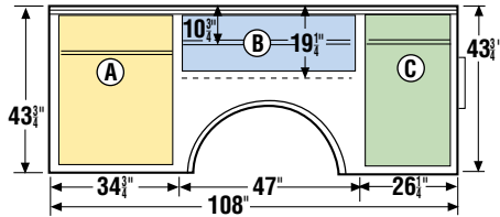
HD108AB "A" Compartment Layout
