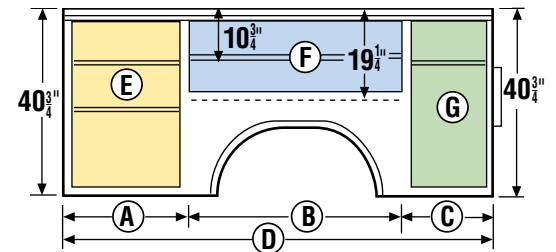
"A" Compartment Layout
