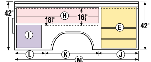
"B" Compartment Layout
